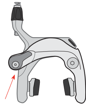
Figure 1. Attachment bolt for front brake quick-release
